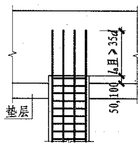
桩顶纵筋在承台内的锚固构造
