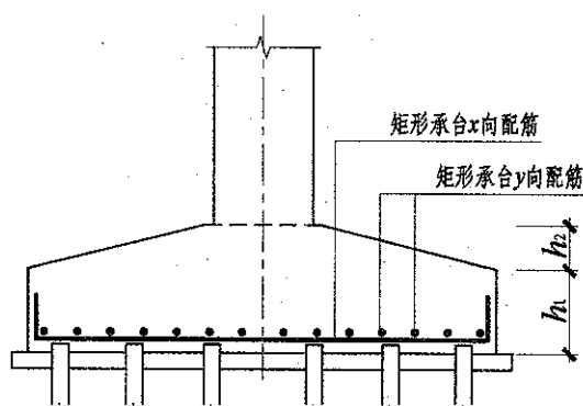
(c) 坡形截面CT p
