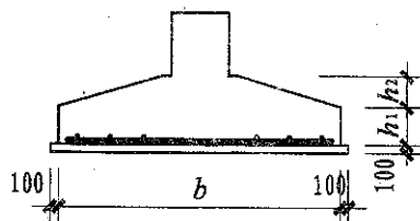
(坡形截面TJB p )
