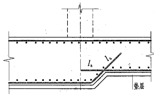
(c) 板底有高差
