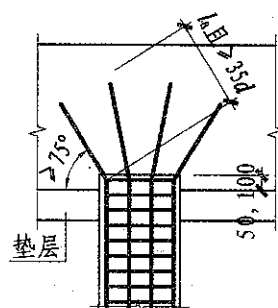
桩顶纵筋在承台内的锚固构造
