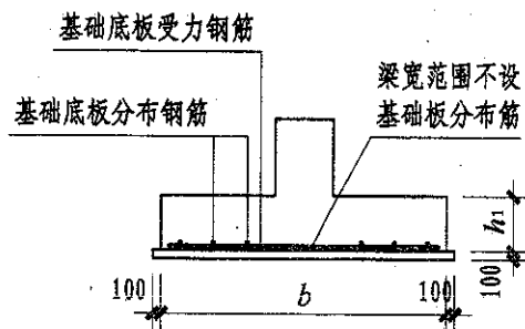
(阶形截面TJB I )
