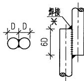
圆钢搭接
