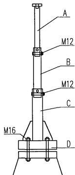
S3000 ,LCT针安装图
