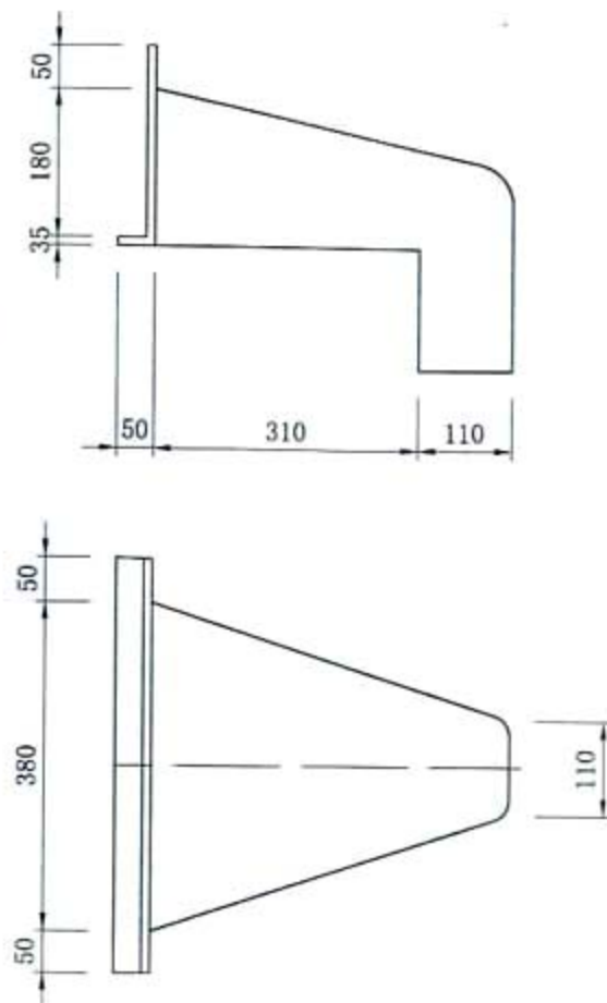
侧向雨水斗 (壁厚3.60)
